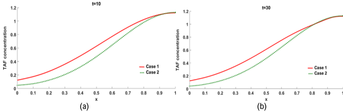
Figure 15: The Concentration of TAFs for Case 1 and Case 2 at Times (a) t = 10 , (b) t = 30
