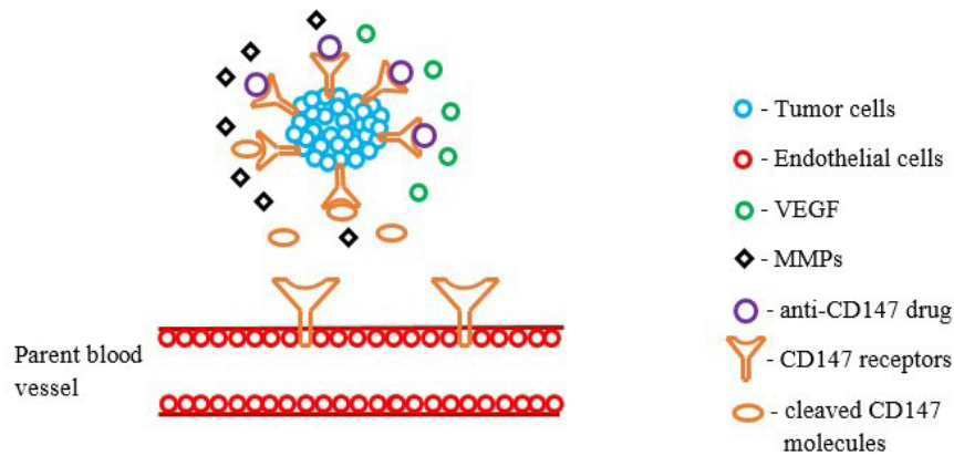
Figure 2: The Action of Anti-CD147 drug
