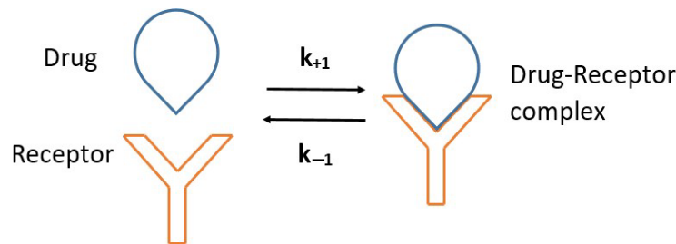
Figure 1: The Drug-Receptor Binding
